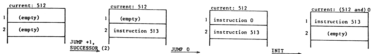
FIGURE 3c: out-of-line execution of instruction 0.
