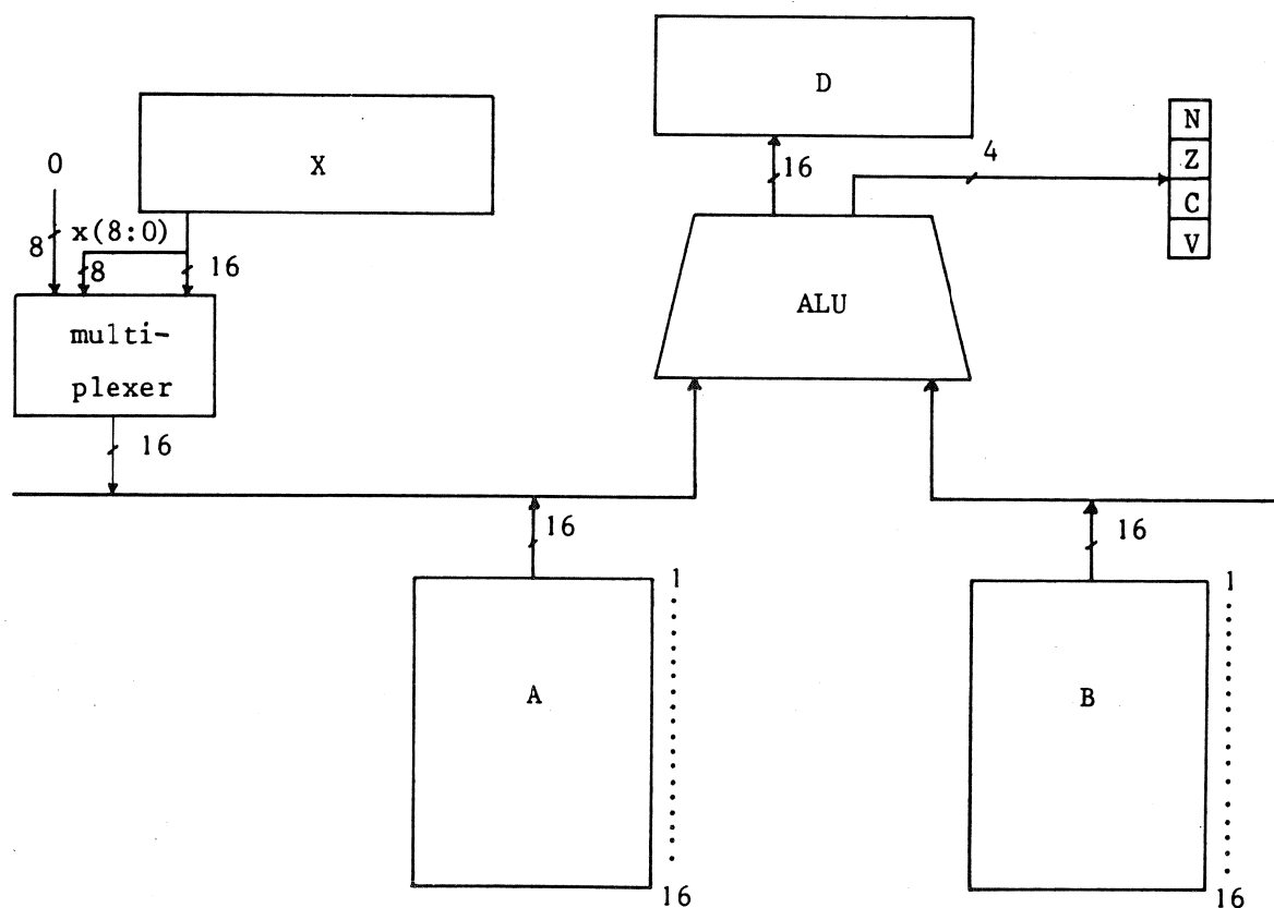
FIGURE 2: Part of the EXMP datapath
